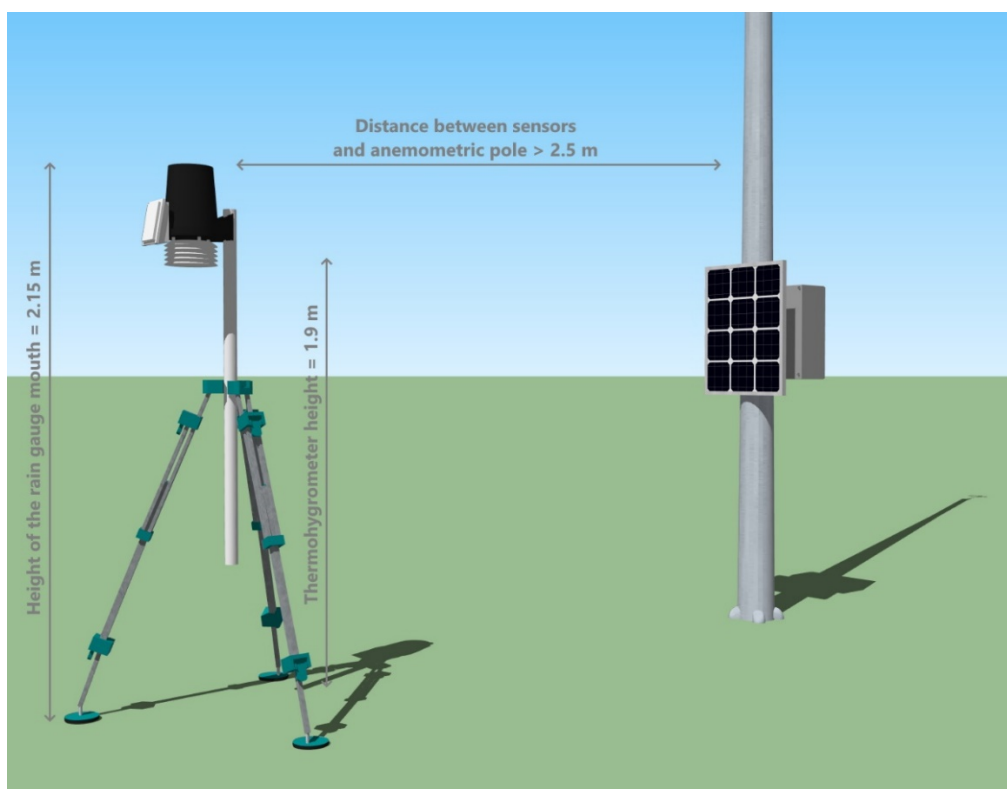
Fig. 9 Examples of indications for installation.
